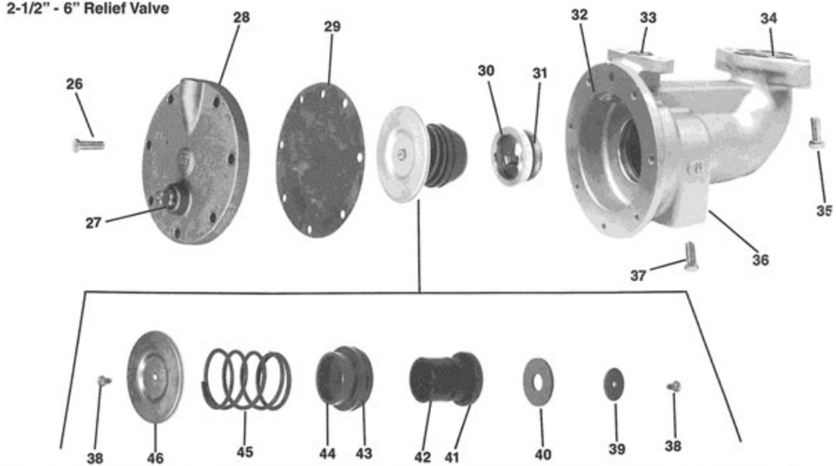
8" & 10" Relief Valve
